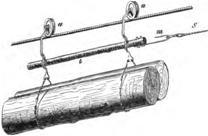
Fig. 225.—Truck for wire-tramway.
